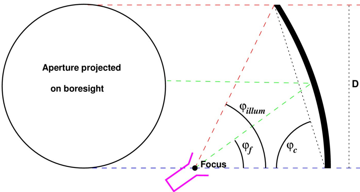
Figure 1 – Offset dish sketch
