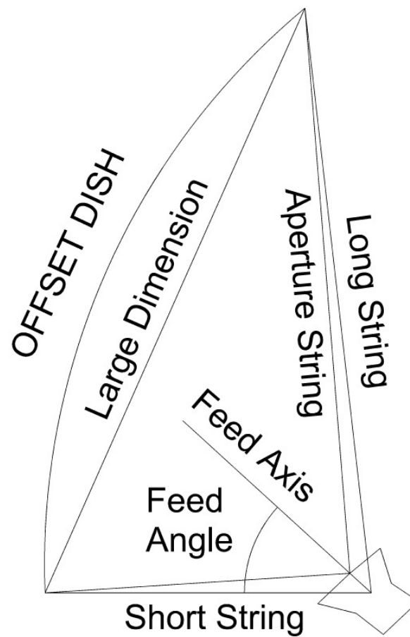
Figure 4 – String lengths to align with center of aperture
