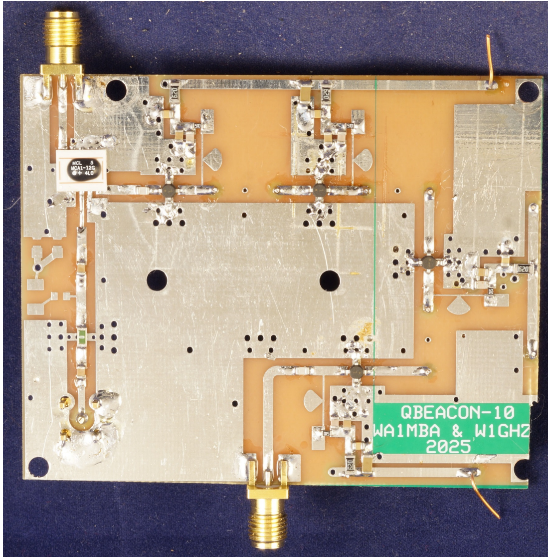
Figure 8 – Qbeacon board for 5760 MHz
